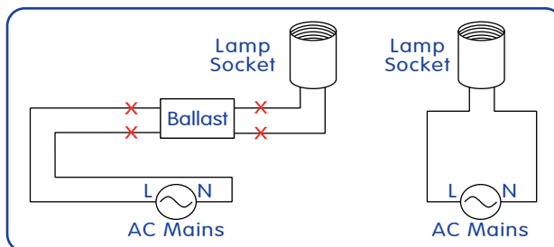
Wiring Diagram for HyLite LED Arc-Cob Lamp (with Internal Driver)
