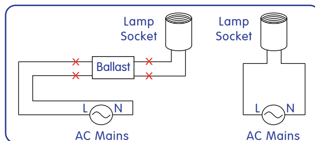
Wiring Diagram for HyLite LED Lotus™ Lamp (with Integrated Driver)
